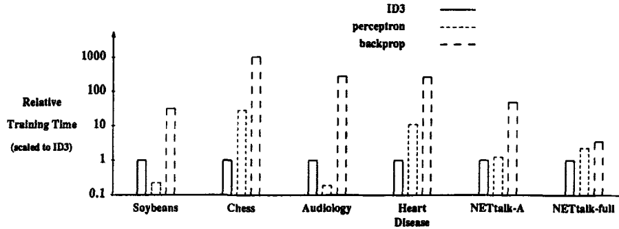
Figure 1. Relative training times of the three algorithms.
