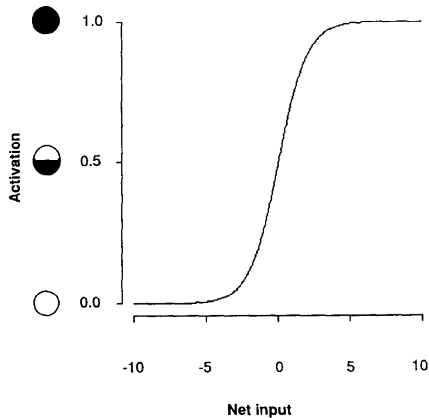
Figure 7. The logistic function used to determine node activations. One term in the weight change equation is the slope of this function; when node activations saturate at either 1.0 or 0.0, this slope asymptotically approaches 0.
