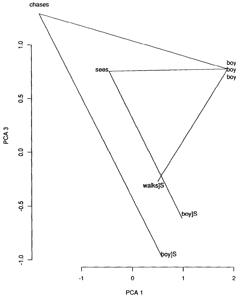
Figure 3. Plot of the movement through two dimensions of hidden unit activation space (first and third principal components) as the network processes the sentences boy chases boy, boy sees boy, and boy walks (sentence endings are indicated with ]S). Nouns occupy the right portion of this plane, and verbs occupy the left side; the axis running from top left to bottom right encodes the verb argument expectations.
